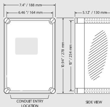
ENCLOSURE
